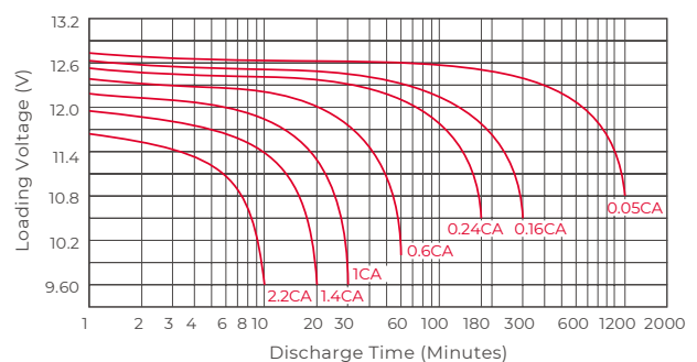
DISCHARGE CHARACTERISTICS
