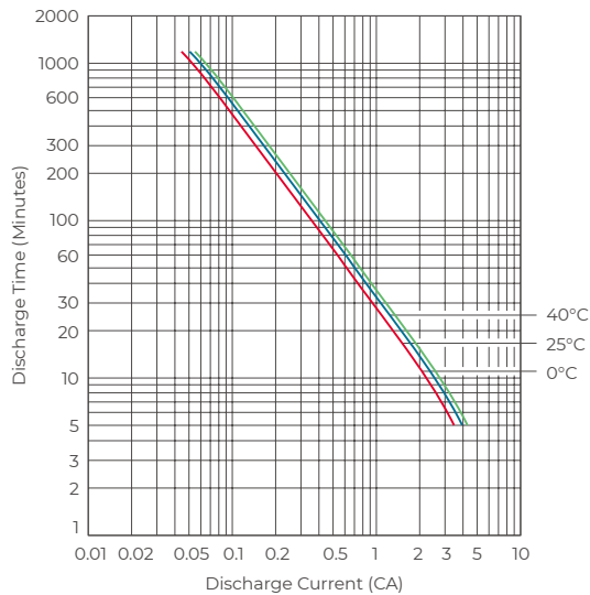
DISCHARGE CURRENT IN RELATION TO DISCHARGE TIME
