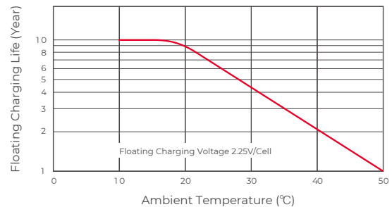
FLOAT CHARGING LIFE CHARACTERISTICS
