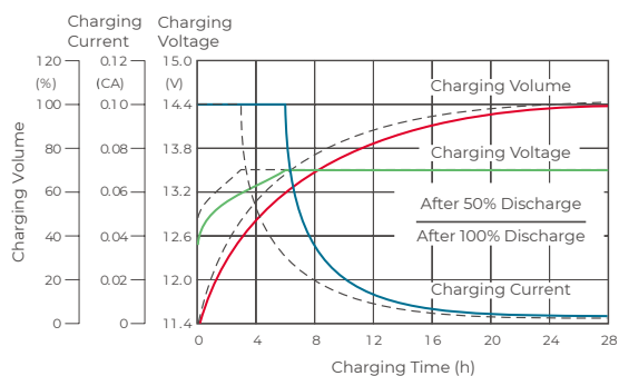
CHARGING CHARACTERISTICS
