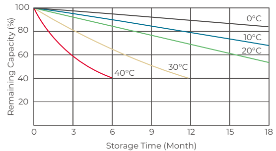
SELF-DISCHARGE CHARACTERISTICS
